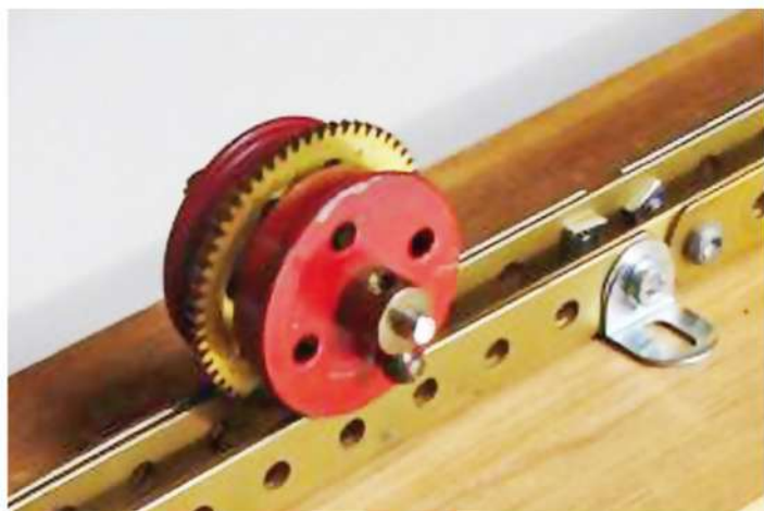
Fig. 14 Rails
