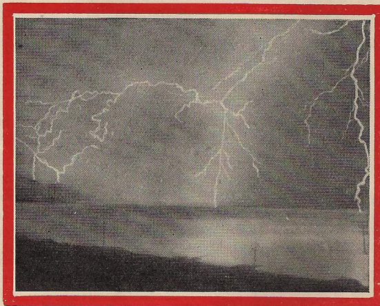
Fig. 39. Flashes of forked lightning, photographed at night.
